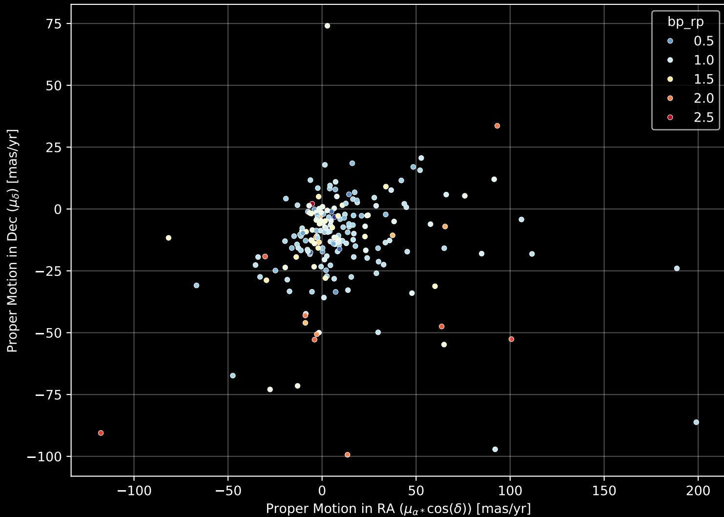
APOGEE DR17 Field: [143-47_MGA] Proper Motion Diagram (n= 201)
