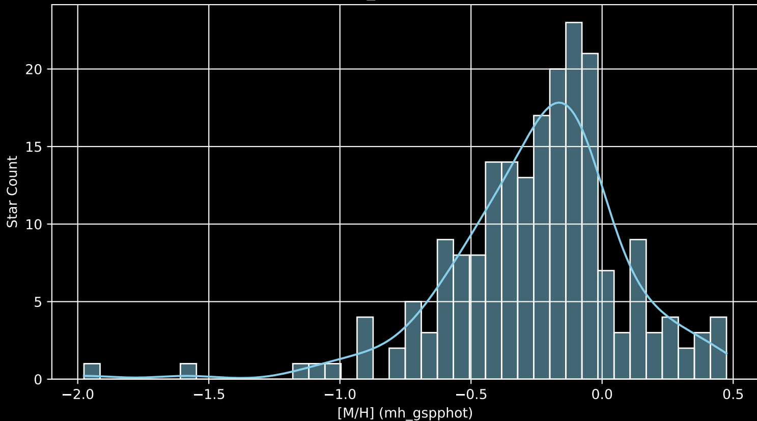
APOGEE DR17 Field: [143-47_MGA [M/H] (mh_gspphot) (n= 201)
