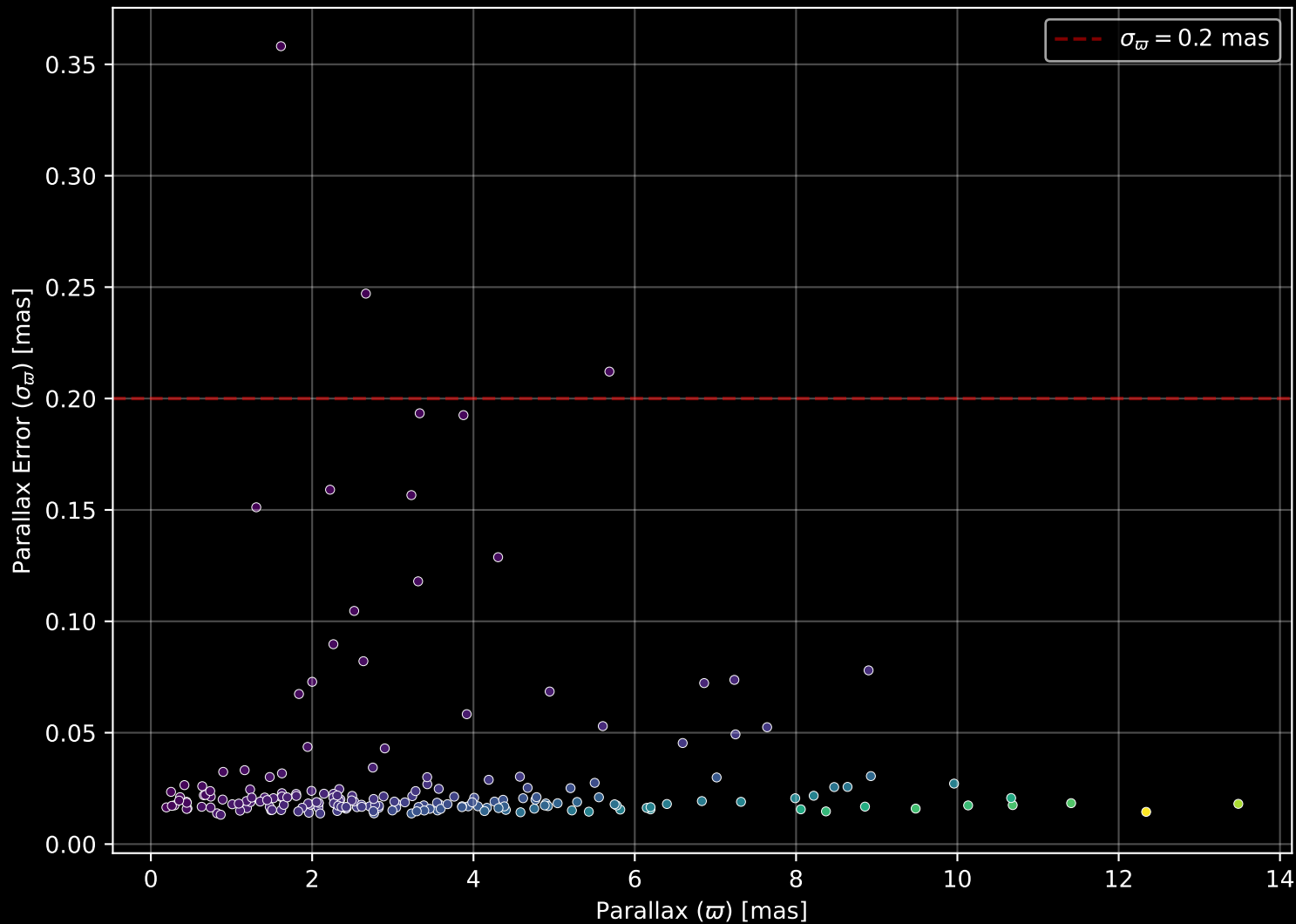
APOGEE DR17 Field: [143-47_MGA] Parallax Quality (n= 201)
