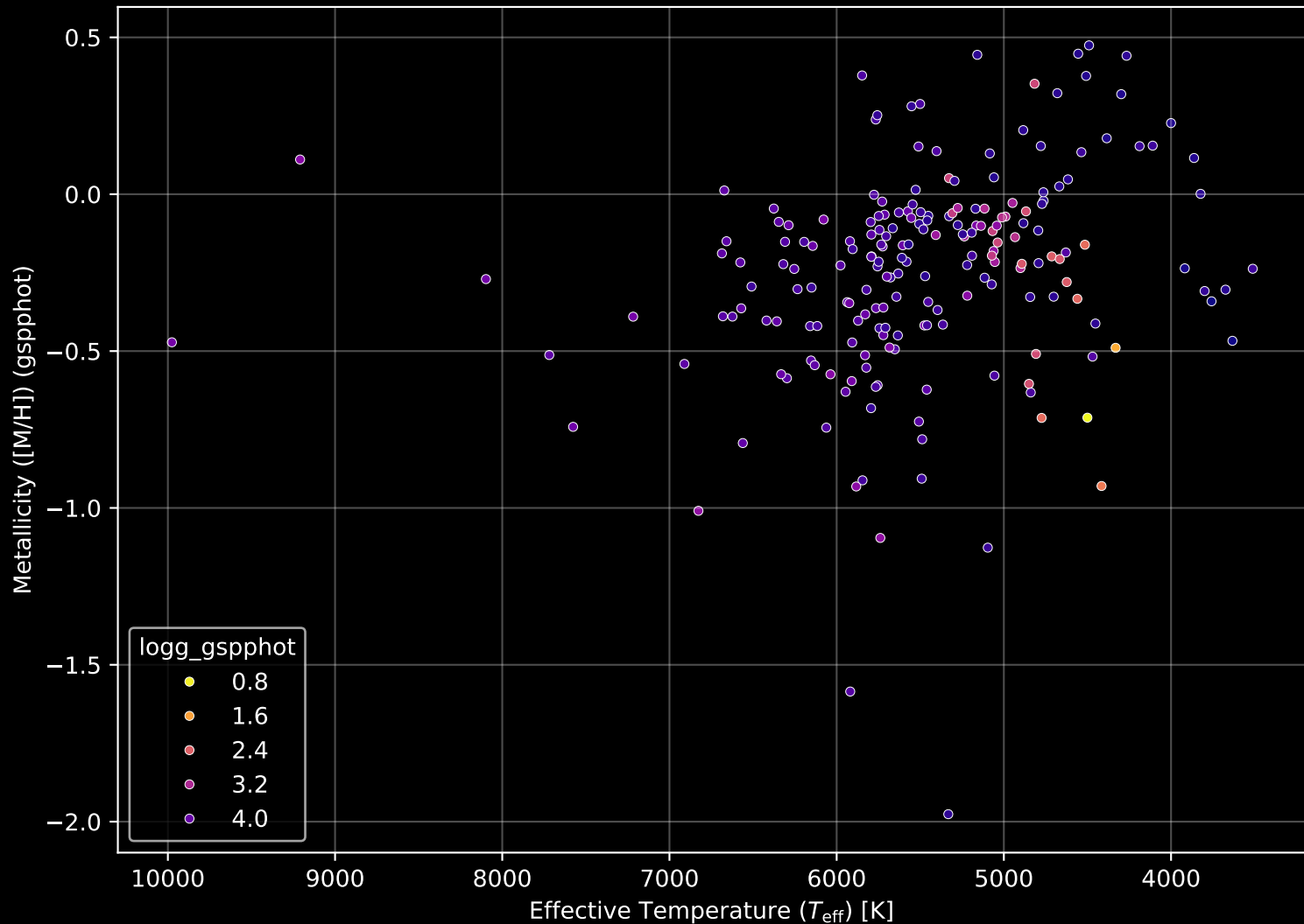
APOGEE DR17 Field: [143-47_MGA] Stellar Population Parameters (n= 201)
