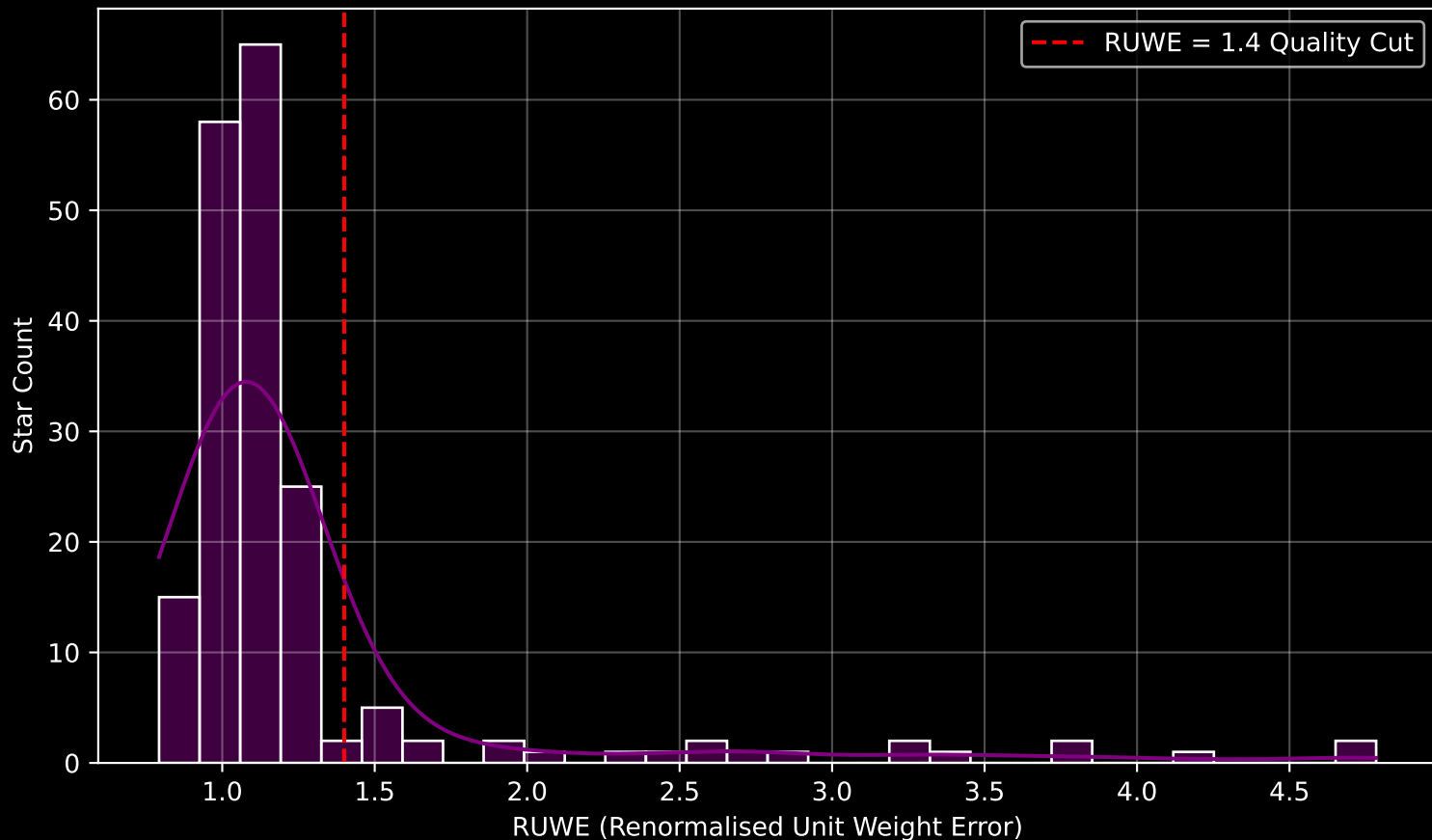
GAPOGEE DR17 Field [143-47_MGA] RUWE Distribution (n= 189)
