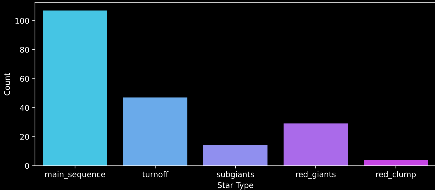
APOGEE DR17 Field: [143-47_MGA] Count plot of Star Type
