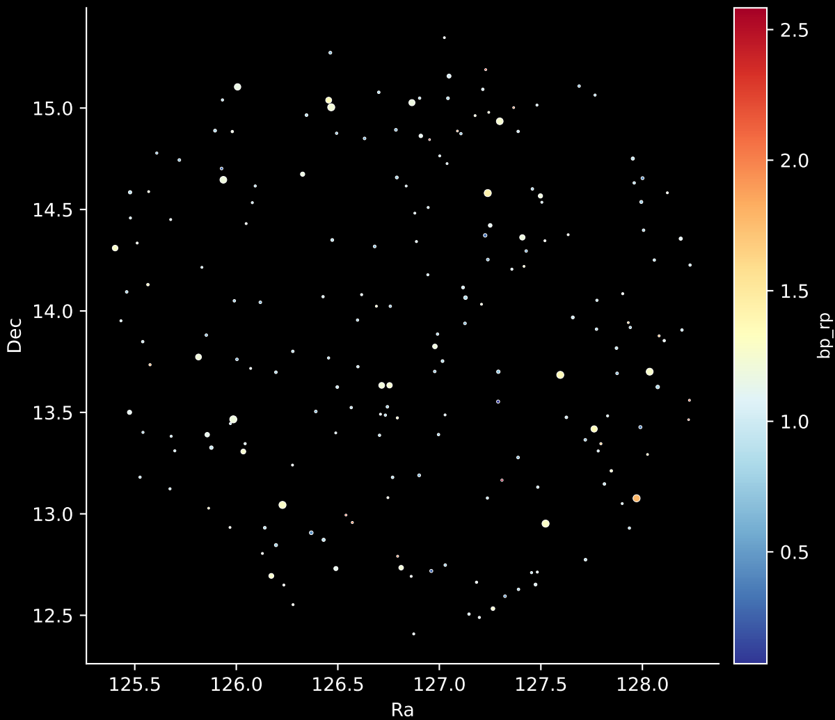
APOGEE DR17 Field: [143-47_MGA] Stars: 201
